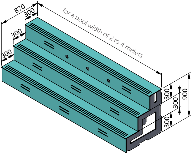
Stairs rectangular 3-stage for depth 1,2 m for a pool width of 2 to 4 meters
