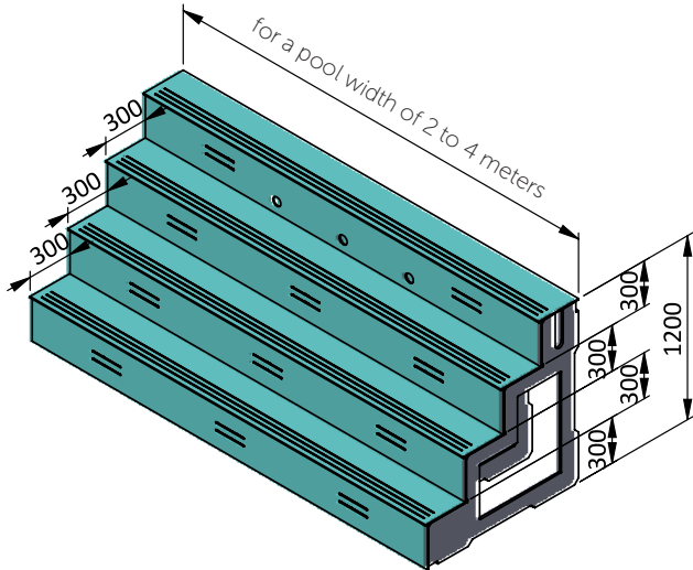
Stairs rectangular 4-stage for depth 1,5 m for a pool width of 2 to 4 meters
