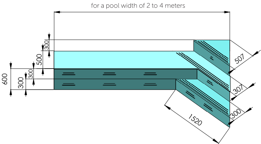
Stairs straight across the corner with a bench 3-stage for depth 1,2 m for a pool width of 2 to 4 meters
