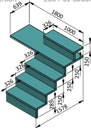
Stairs X-AIR PLUS 5-stage for depth 1,5 m right version: 2B04-01-SD077 left version: 2B04-01-SD087
