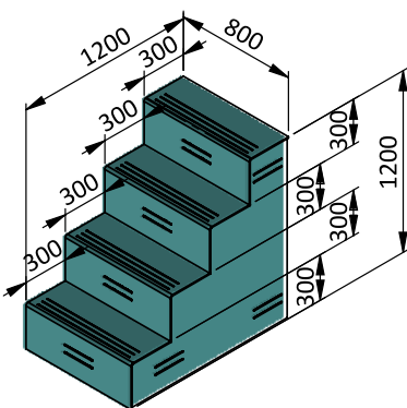
Stairs rectangle in the corner of 4-step for depth 1,5 m right version: 2B04-01-SD129 left version: 2B04-01-SD130
