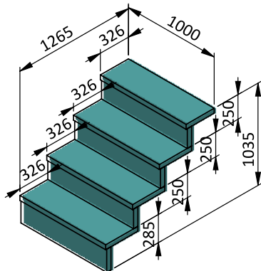
Stairs X-AIR 4-stage for depth 1,2 m right version: 2B04-01-SD084 left version: 2B04-01-SD074
