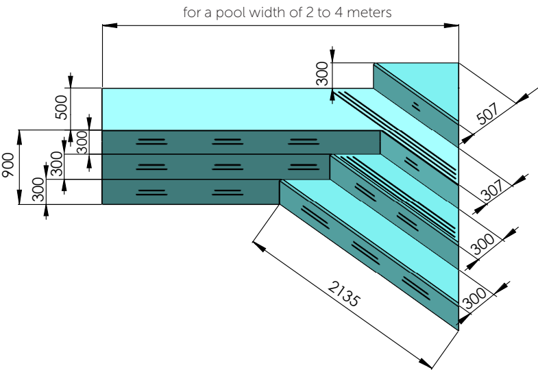
Stairs straight across the corner with a bench 4-stage for depth 1,5 m for a pool width of 2 to 4 meters
