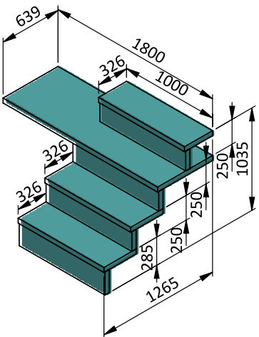
Stairs X-AIR PLUS 4-stage for depth 1,2 m right version: 2B04-01-SD076 left version: 2B04-01-SD086
