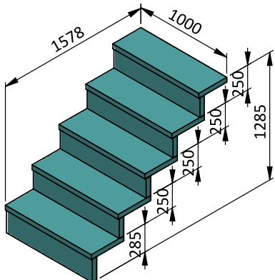
Stairs X-AIR 5-stage for depth 1,5 m right version: 2B04-01-SD085 left version: 2B04-01-SD075
